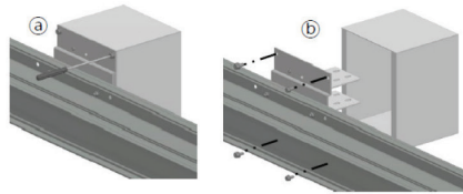
Figure 34. Busway Pre-installation
