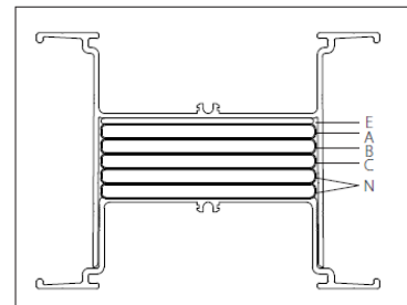
[3P5W(200%N)+50%E+GE]
