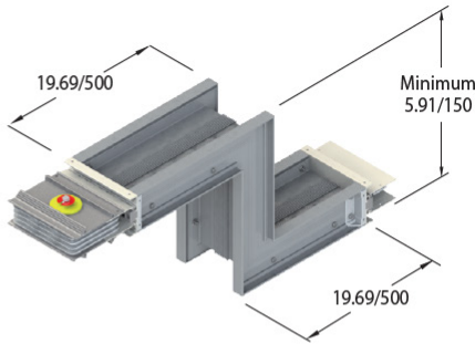
Offset [Horizontal Edgewise Orientation]
