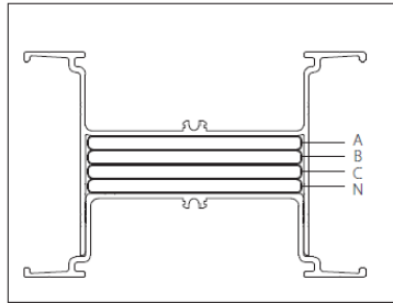
[3P4W(100%N)+GE]
