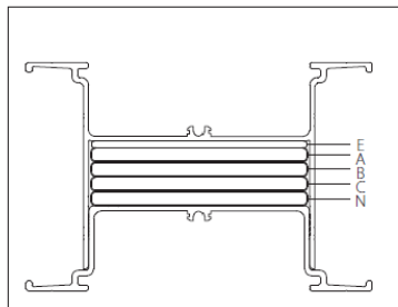
[3P4W(100%N)+50%E+GE]
