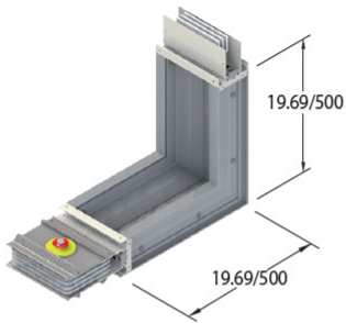
Elbow [Horizontal Edgewise Orientation]
