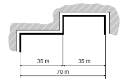
Section length 70 m. When the section is not straight, no expansion element is necessary
