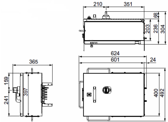
Type 2 (250A) – MCCB ready (removable cover)
