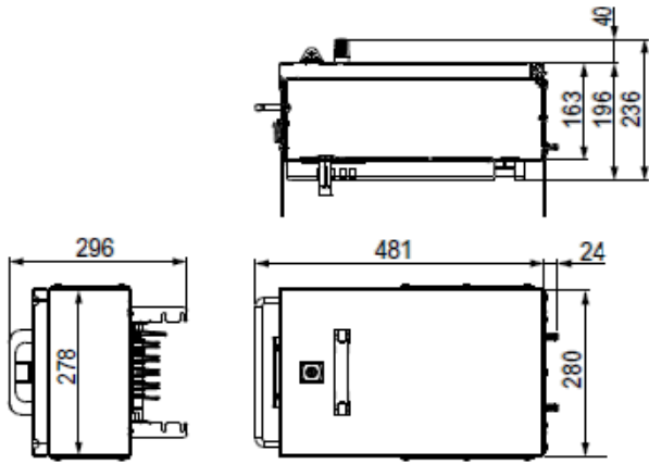
Type 1 (63A / 125A / 160A) – empty
