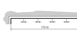
Straight section length 170 m: no. 4 expansion elements, one every 34 m
