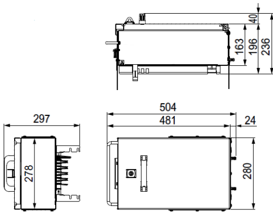
Type 1 – total dimensions with cover open
