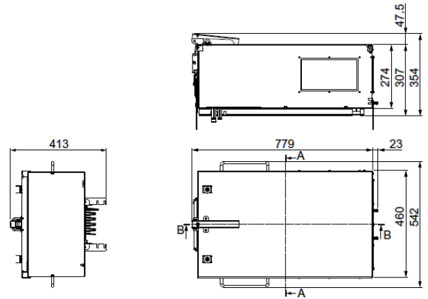
Type 3 - total dimensions with cover open
